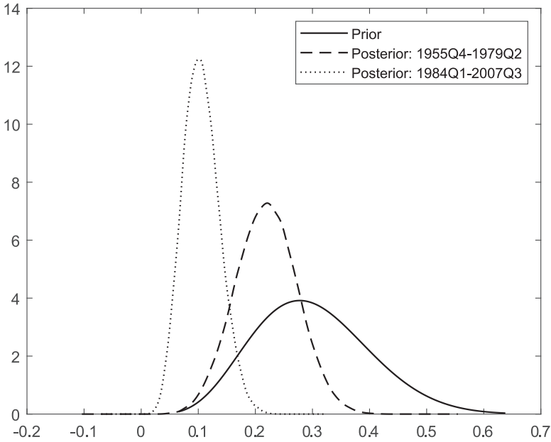
Fig. 2. Prior-Posterior Plot for \theta .
