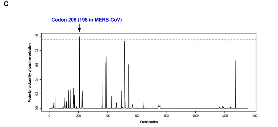
Figure 1. Positive selection at the spike gene of MERS-CoV-related coronaviruses. (A) Cartoon representation of the MERS-CoV spike protein with distinct domains in different colors (SP, signal peptide; NTD, N-terminal domain; RBD, receptor binding domain; FP, fusion peptide; HR1 and HR2, heptad repeat 1 and 2; TM, transmembrane domain; CP, cytoplasmic domain). The location of positively selected sites detected in MERS-CoV related sequences is shown in red. A positively selected residue in MERS-CoV isolated from humans and camels is shown in orange. The positively selected site and recombination breakpoints in Pi-BatCoV HKU5 sequences are shown in blue and black, respectively. Furin cleavage sites are depicted as triangles 56 . Two alignment portions are shown; positions that alter virus host range or tropism in SARS-CoV, MHV, and Beaudette strain IBV (IBV Beau CK) are highlighted in green 25–27 . A functional mutation which arose during tissue-culture adaptation of MERS-CoV (strain EMC2012) is highlighted in grey 31 . (B) Bayesian phylogenies for the S1 (left) and S2 (right) sequences 6 ; branch length is proportional to dS. Branches in red were set as foreground lineages in independent branch-site tests. Thick branches yielded statistically significant evidence of positive selection. The bracket denotes a subset of sequences that were used for analysis of positive selection in the RBD. (C) OmegaMap results for Pi-BatCoV HKU5 spike genes. The hatched red line corresponds to a posterior probability of selection equal to 0.95.
