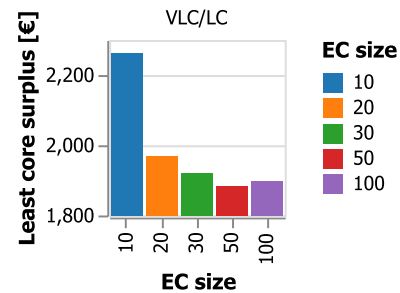
Fig. 6. Community surplus ( \theta^{LC} ) by EC size - precoalitions [1, |J|] .
