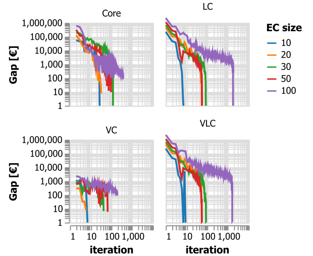
Fig. 5. Convergence characteristics of the iterative techniques - precoalitions [1, |J|] ; tolerance is 1-100€ (about 1-5%).
