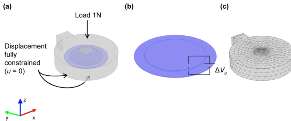
Figure 2. Finite element method (FEM) model of the encapsulated transducer. (a) Schematic of the actuator showing the boundary conditions on the PDMS structure; (b) detail of the piezoelectric disk showing the driving voltage imposed on the element; and (c) a view of the meshed geometry of the whole encapsulated transducer.
