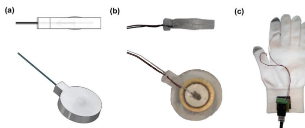
Figure 6. Embedded piezoelectric transducer. (a, upper part) Drawing of the lateral view of the piezoelectric transducer embedded in the polymeric matrix, with evidence of the two protrusions on the external opposite faces of the geometry; (a, lower part) drawing of the upper view of the piezoelectric transducer embedded in the polymeric matrix; (b, upper part) lateral picture of the developed prototype showing the side of the actuator; (b, lower part) upper picture of the developed prototype showing the whole surface of the actuator; and (c) a picture of the integrated system used for the psychophysical evaluation: a textile glove equipped with two encapsulated transducers on the thumb and index fingertips.
