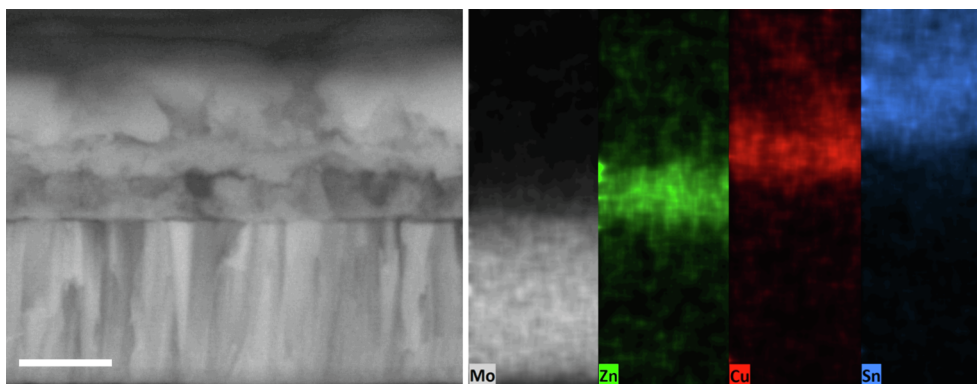
Fig. 4. SEM [scale bar: 500 nm] and elemental mapping of the fractured cross-section of Mo/Zn/Cu/Sn stack.
