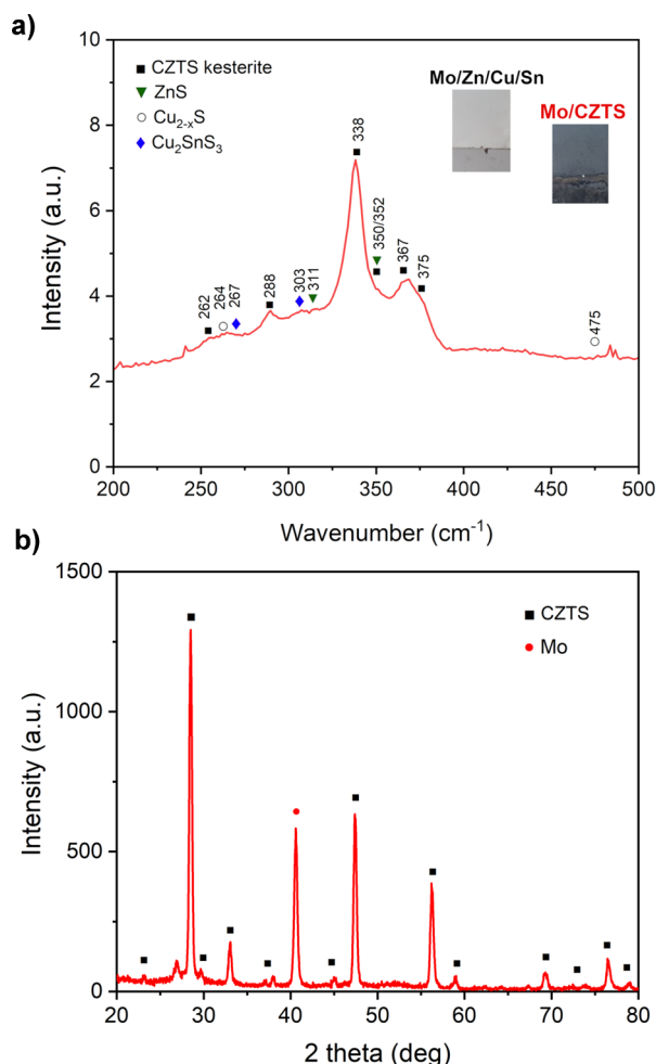
Fig. 5. CZTS film after soft and reactive annealing of the Zn/Cu/Sn stack in a sulfur atmosphere (a) Raman spectrum (b) XRD spectrum.
