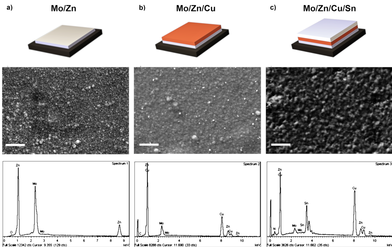
Fig. 3. SEM [scale bar: 3 μm] of the sample surface, EDS and graphical representation of the CZT metallic stack. (a) Mo/Zn; (b) Mo/Zn/Cu; (c) Mo/Zn/Cu/Sn.
