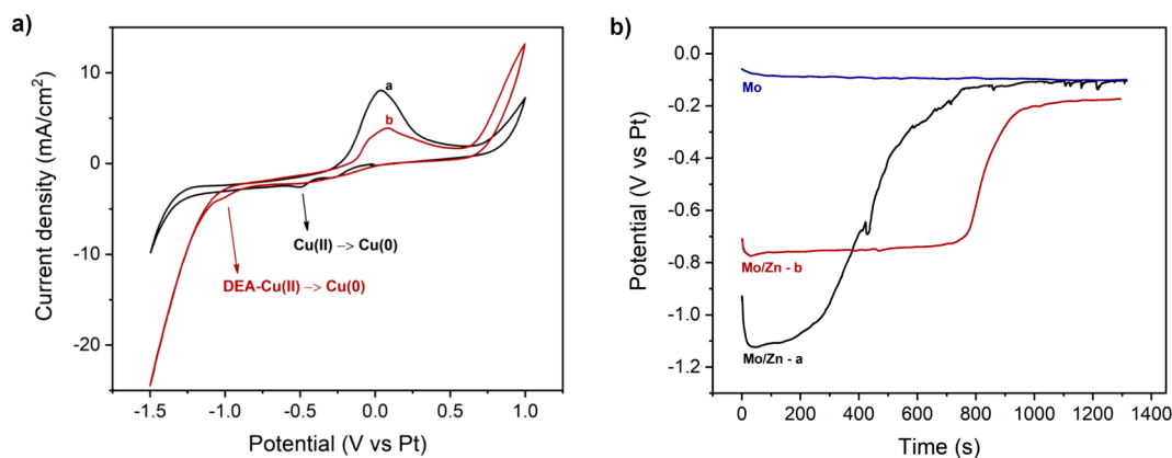
Fig. 1. (a) Cyclic voltammetry (T 70 °C, 20 mV/s) on GC electrode of 0.05 M copper acetate, 1 M sodium acetate in ethylene glycol (curve a) and with the addition of 0.8 M DEA (curve b). (b) Copper displacement investigation (OCV-time graph) of Mo/Zn substrate immersed in a copper 0.05 M copper acetate, 1 M sodium acetate in ethylene glycol (curve a) and with the addition of 0.8 M DEA (curve b) at 70 °C.
