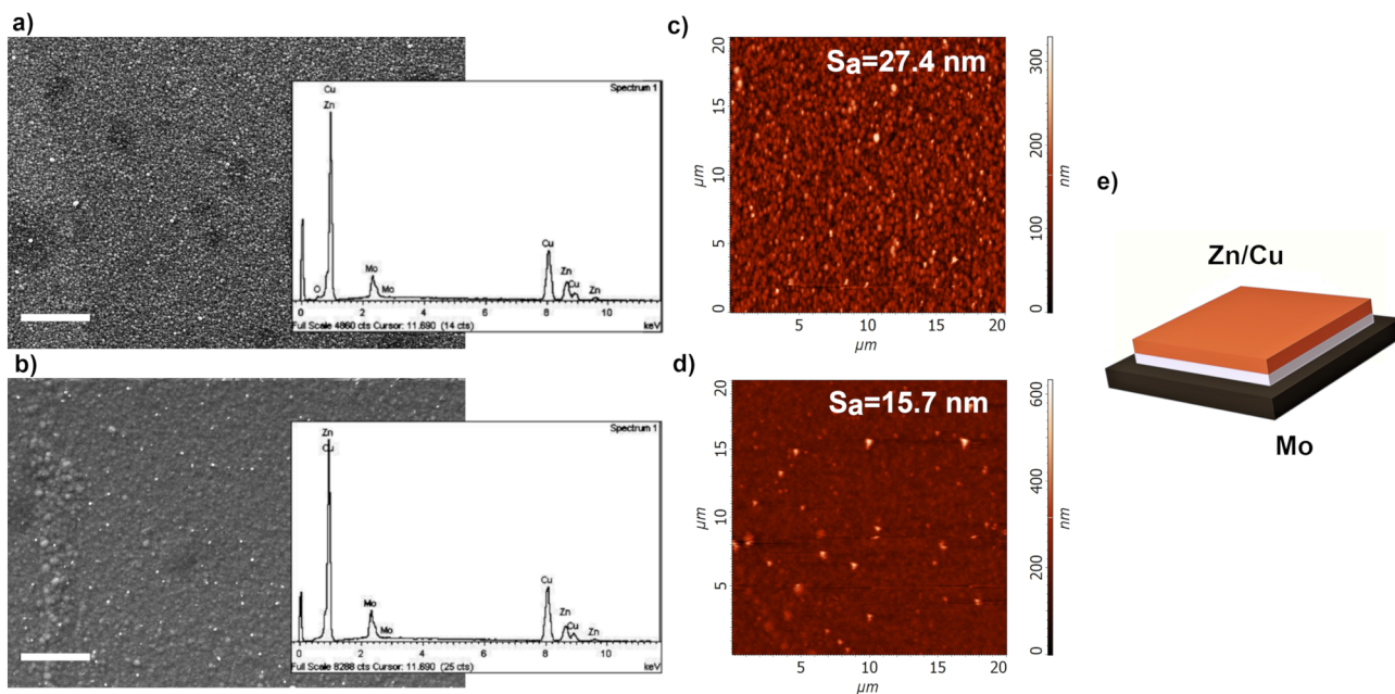
Fig. 2. SEM [scale bar: 5 \mu\text{m} ], EDS and AFM analysis of copper layer onto zinc (a, c) -2 \text{ mA/cm}^2 , 70 °C, DEA-free solution. (b, d) -2 \text{ mA/cm}^2 , 70 °C, DEA-containing solution. (e) Graphical representation of the Zn/Cu stack.
