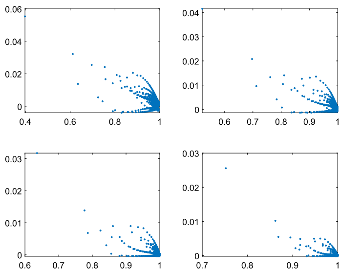
Fig. 10. Eigenvalues of the preconditioned matrix of size n^2 = 2^{12} for \mu(x, y) = -2 + \exp(i(3x + 2y)) , and \alpha = \{1.2, 1.4, 1.6, 1.8\} , respectively.
