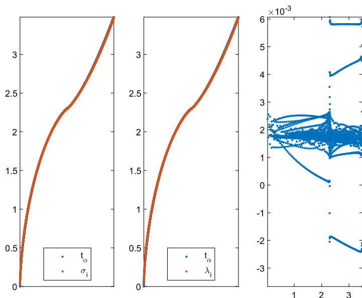
Fig. 1. Singular/Eigenvalues of the matrix \hat{A}_{\mathbf{n}} for \mu(x, y) = \exp(i(x + 4y)) , \alpha = 1.2 and n^2 = 2^{12} . The first (second) panel reports in blue the singular values (real part of the eigenvalues) and in red the equispaced sampling of t_{\alpha} in nondecreasing order. The third panel reports the eigenvalues in the complex plane. (For interpretation of the colors in the figure(s), the reader is referred to the web version of this article.)
