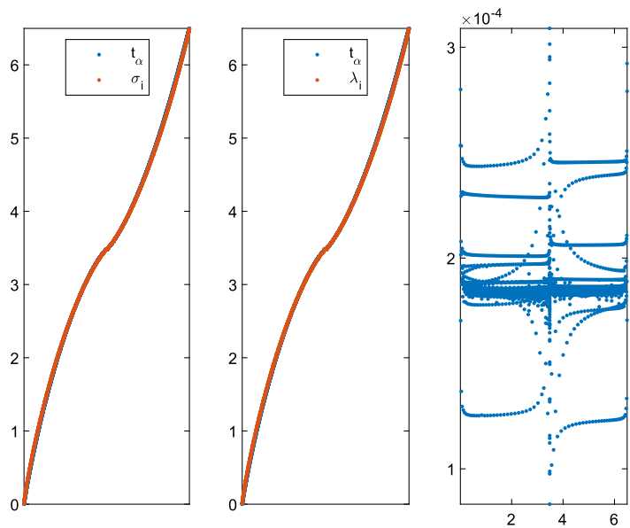
Fig. 8. Singular/Eigenvalues of the matrix \hat{A}_n for \mu(x, y) = -2 + \exp(i(3x + 2y)) , \alpha = 1.8 and n^2 = 2^{12} . The first (second) panel reports in blue the singular values (real part of the eigenvalues) and in red the equispaced sampling of t_\alpha in nondecreasing order. The third panel reports the eigenvalues in the complex plane.
