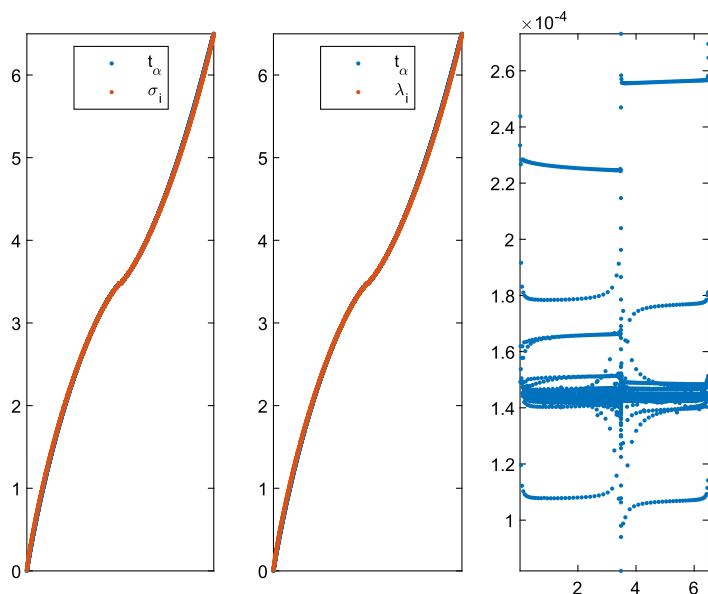
Fig. 4. Singular/Eigenvalues of the matrix \hat{A}_n for \mu(x, y) = \exp(i(x + 4y)) , \alpha = 1.8 and n^2 = 2^{12} . The first (second) panel reports in blue the singular values (real part of the eigenvalues) and in red the equispaced sampling of t_\alpha in nondecreasing order. The third panel reports the eigenvalues in the complex plane.
