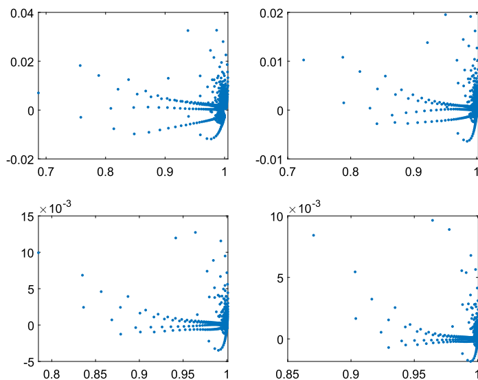
Fig. 9. Eigenvalues of the preconditioned matrix of size n^2 = 2^{12} for \mu(x, y) = \exp(i(x + 4y)) and \alpha = \{1.2, 1.4, 1.6, 1.8\} , respectively.
