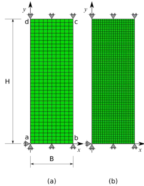
Figure 17. Biaxial tests: problem geometry and finite element discretizations adopted. a) Coarse mesh, 10 \times 35 Q4 elements; b) fine mesh, 20 \times 70 Q4 elements.
