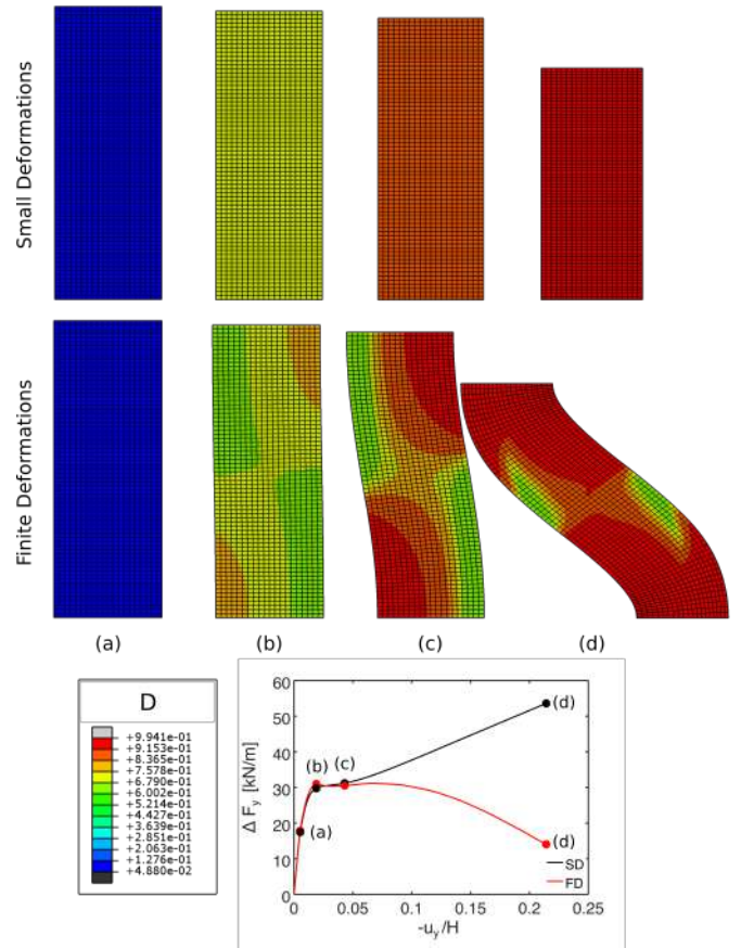
Figure 24. Biaxial tests bx004 and bx104: Contour maps of damage index D at different time stations.
