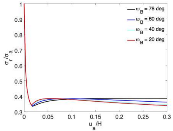
Figure 14. Oedometric compression tests ax101–ax103: effect of \omega_B on the evolution of \sigma_r/\sigma_a .
