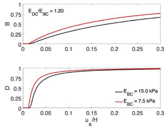
Figure 11. Oedometric compression tests ax101–ax102: effect of E_{BC} and E_{DC} on the evolution of breakage and damage indices.
