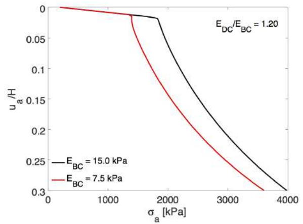
Figure 10. Oedometric compression tests ax101–ax102: effect of E_{BC} and E_{DC} on the compressibility curves.
