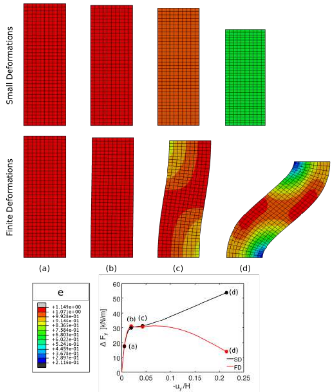
Figure 26. Biaxial tests bx002 and bx102: Contour maps of void ratio e at different time stations, coarse mesh.
