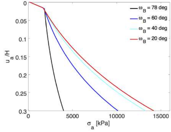
Figure 13. Oedometric compression tests ax101–ax103: effect of \omega_B on the compressibility curves.
