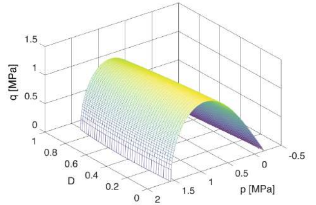
Figure 3. Yield function in (p, q, D) space for B = 0.0 . Material constants from Set 1 of Tab. 1.
