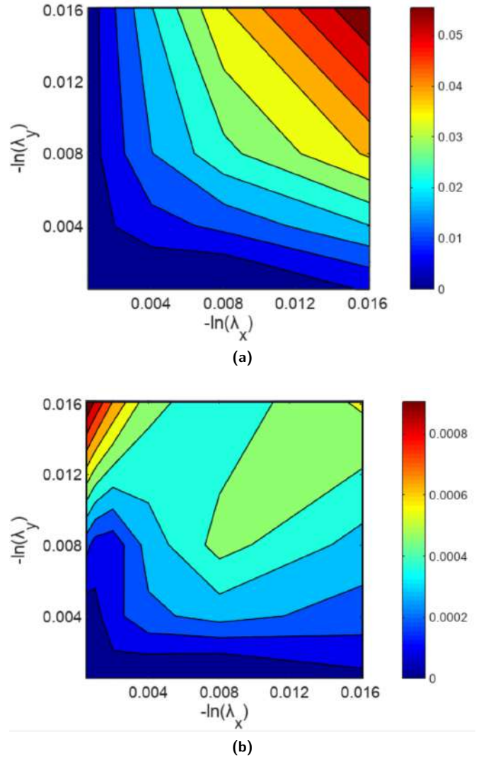
Figure 15. Isoerror maps: a) \text{ERR}_\sigma ; b) \text{ERR}_q .
