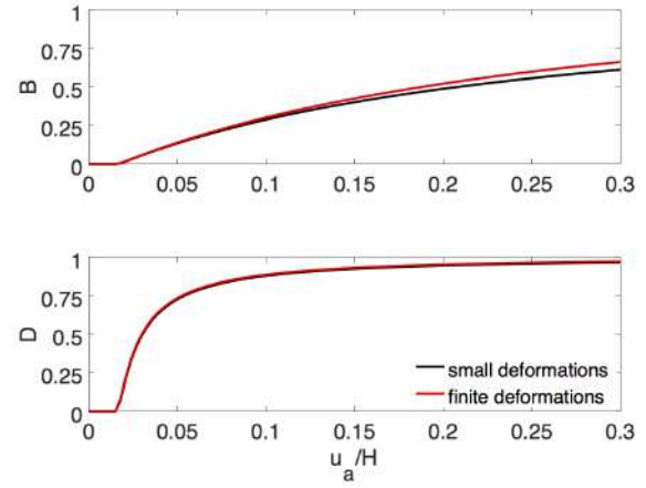
Figure 9. Oedometric compression tests ax001–ax101: evolution of breakage and damage indices for small and finite deformations.
