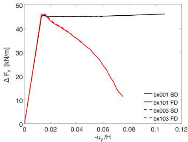
Figure 18. Biaxial tests at low confining stress: axial load increment \Delta F_y vs. normalized axial shortening -u_y/H .
