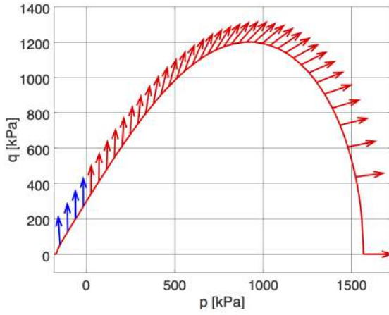
Figure 4. Yield function in (p, q) space for B = 0.0 and D = 0.0 . Arrows provide the local direction of the plastic flow. Contractant flow is represented with red arrows, dilatant flow with blue arrows. Material constants from Set 1 of Tab. 1.
