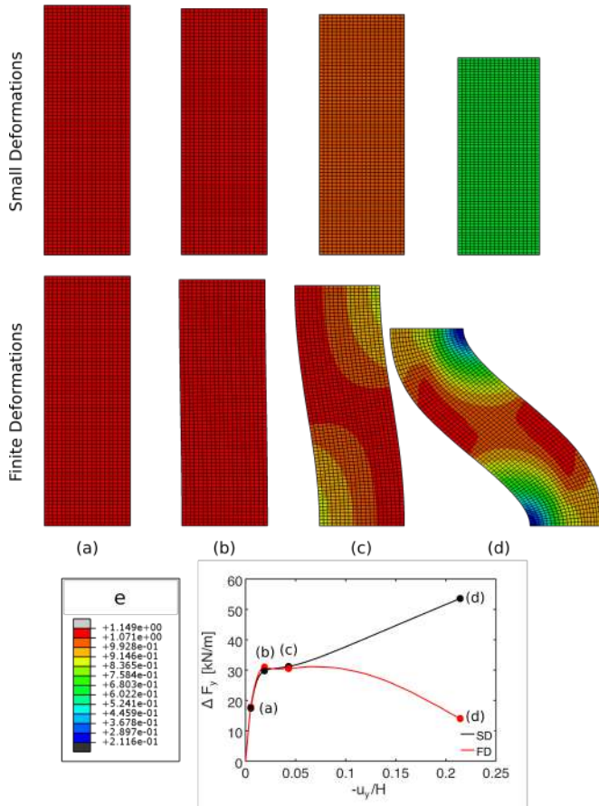
Figure 25. Biaxial tests bx004 and bx104: Contour maps of void ratio e at different time stations.
