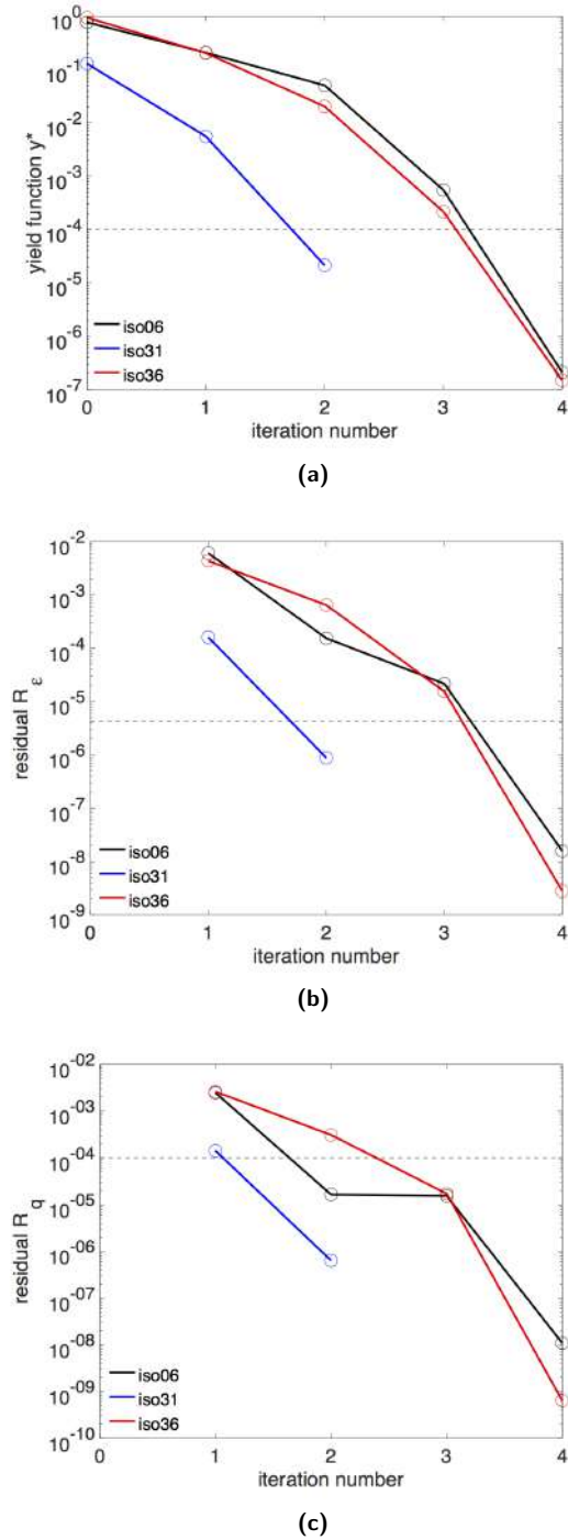
Figure 16. Convergence profiles for simulations iso06, iso31 and iso36: a) yield function y^* ; b) residual R_\epsilon ; c) residual R_q .
