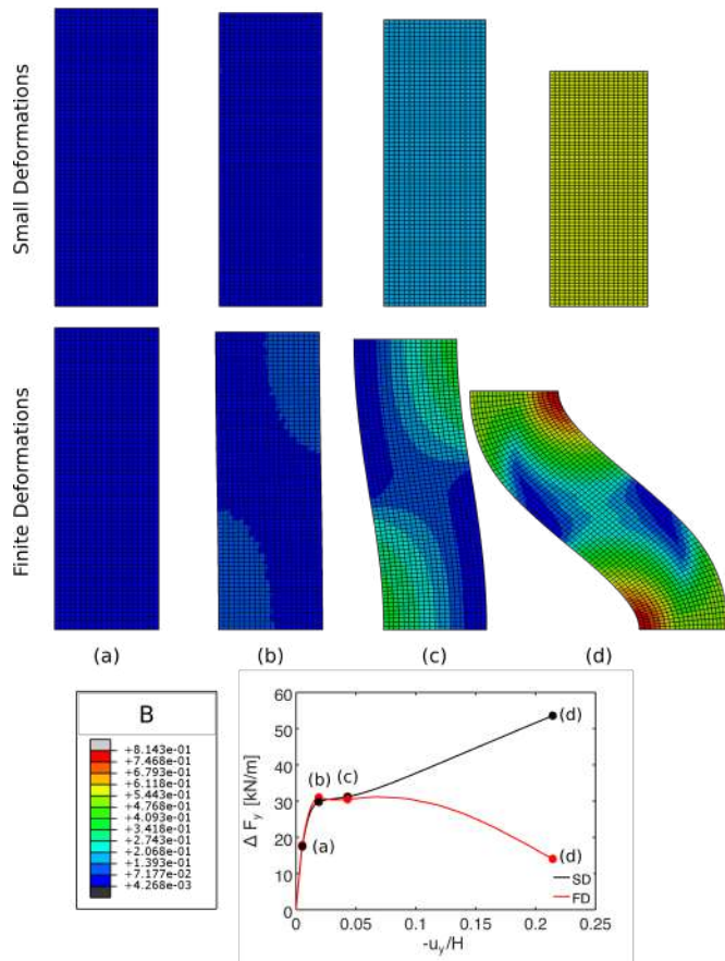
Figure 23. Biaxial tests bx004 and bx104: Contour maps of breakage index B at different time stations.
