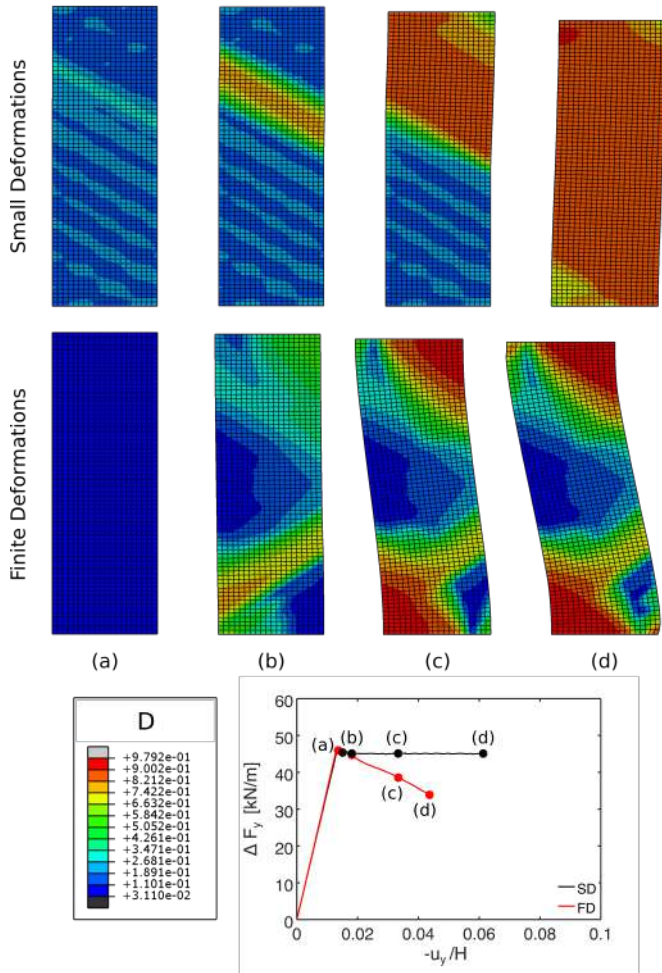
Figure 20. Biaxial tests bx003 and bx103: Contour maps of damage index D at different time stations.
