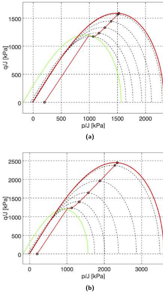
Figure 8. Oedometric compression tests ax001–ax101: stress paths for a) small deformations; b) finite deformations.
