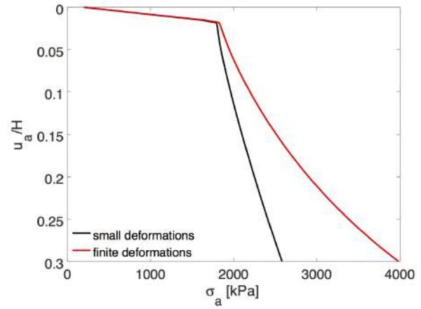
Figure 7. Oedometric compression tests ax001–ax101: compressibility curves for small and finite deformations.
