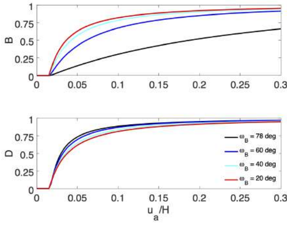
Figure 12. Oedometric compression tests ax101–ax103: effect of \omega_B on the evolution of breakage and damage indices.
