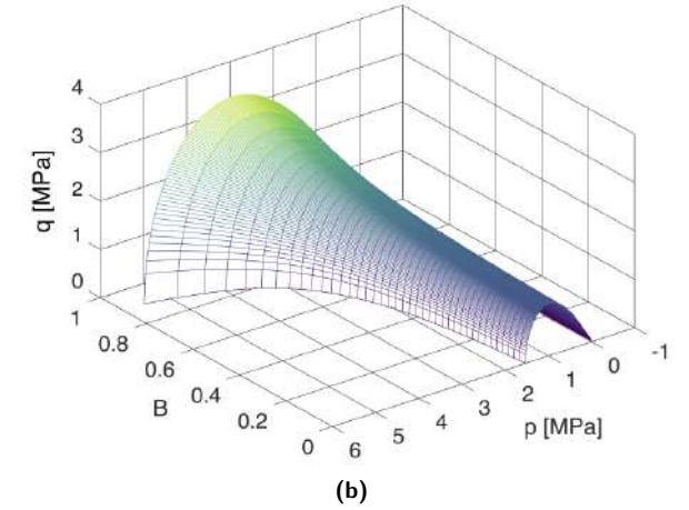
Figure 2. Yield function in (p, q, B) space: a) D = 0.1 ; b) D = 0.9 . Material constants from Set 1 of Tab. 1.
