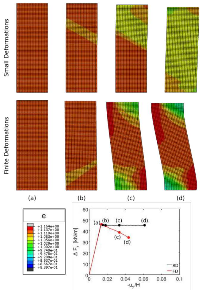
Figure 21. Biaxial tests bx003 and bx103: Contour maps of void ratio e at different time stations.
