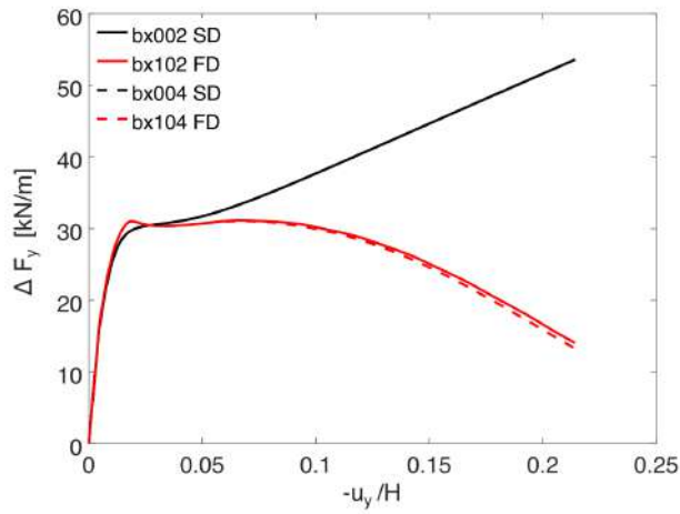
Figure 22. Biaxial tests at high confining stress: axial load increment \Delta F_y vs. normalized axial shortening -u_y/H .
