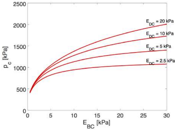
Figure 5. Effect of critical breakage and bond damage energies on isotropic yield stress p_c , for B = 0.0 and D = 0.1 . Material constants from Set 1 of Tab. 1.
