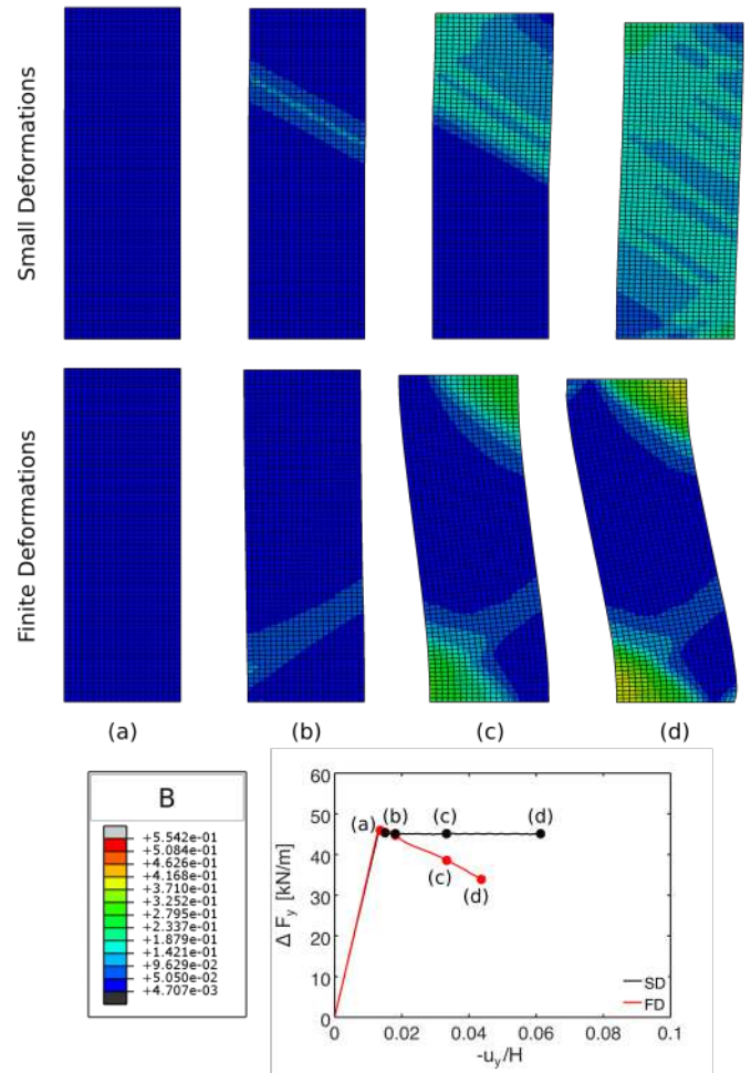
Figure 19. Biaxial tests bx003 and bx103: Contour maps of breakage index B at different time stations.
