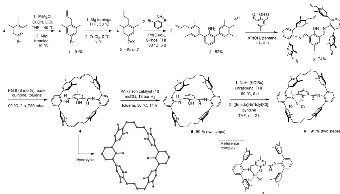
Scheme 1. Synthesis scheme for an N,O -coordinated \text{Ni}^{\text{II}} phenoxydiimine cyclophane complex ( 6 ). The solid-state structure of a hydrolysis product of 4 [15] is also shown, and a non-bridged reference complex ( 7 ).
