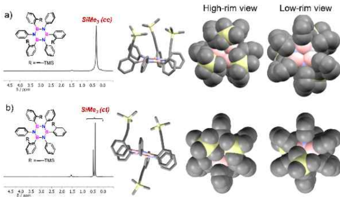
Figure 4. 400-MHz 1 H-NMR in CDCl 3 and single-crystal X-ray structures of a) cc-9 (P2 1 ), b) ct-9 (Pna2 1 ), with ct-9 obtained by heating a solution of cc-9 . Crystals were grown by slow diffusion of i PrOH in either CHCl 3 or CH 2 Cl 2 with those of cc-9 obtained at 4–11 °C to avoid isomerization. Grey: C, pink: B, blue: N and yellow: Si.
