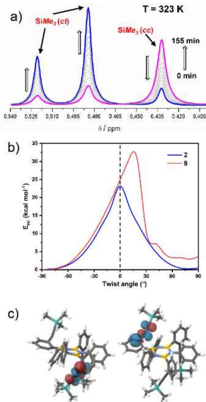
Figure 5. a) Time-dependent ^1\text{H} NMR investigations of the cc \rightarrow ct isomerization at 50^\circ\text{C} . b) Isomerization energy diagram for the cc \rightarrow ct transformations for molecules 2 and 9 as a function of the \text{N}-\text{B}-\text{C}-\text{C} dihedral angle (structures optimized with a fixed \text{N}-\text{B}-\text{C}^1-\text{C}^2 angle in steps of 10^\circ starting from -90^\circ ). c) Borazine 9 corresponding to the energy maximum upon twisting one alkynylphenyl ring, showing the donor-acceptor interactions associated with delocalization about the alkyne (left) perpendicular and (right) parallel to the borazine core obtained at the [B3LYP | 6-31 + G(d,p)] level of theory.
