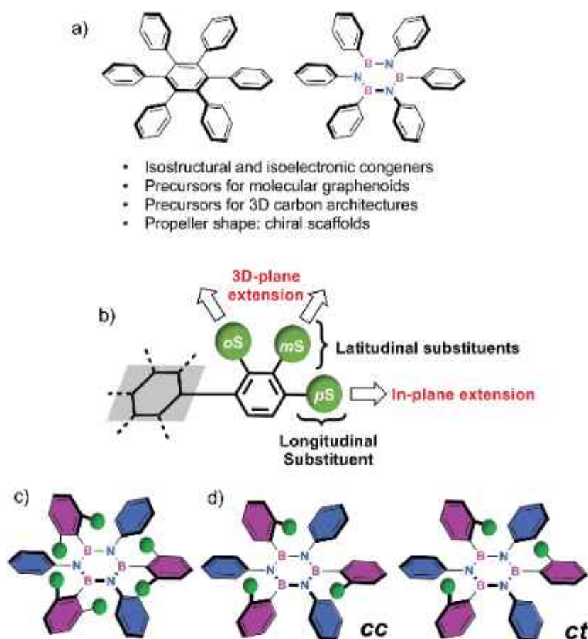
Figure 1. a) Chemical structure of unsubstituted HABs and HABNs. b) Latitudinal ( oS and mS ) and longitudinal ( pS ) substituents allowing the 3D and 2D extension. c) Hexa- oS -aryl borazine. d) Tri- oS -aryl borazine cc and ct stereoisomers. mS : meta-, pS : para-, and oS : ortho- substituent; c : cis , and t : trans .
