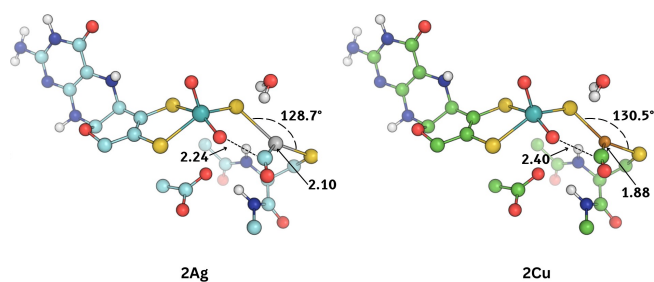
Figure 3. Graphical representation of the optimised intermediates 2Ag and 2Cu . Colour code for 2Ag as in Figure 2. Color code for 2Cu : Mo, cyan; Cu, copper; S, yellow; O, red; N, blue; C, green; H, white. The most representative distances are reported in Å.
