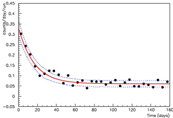
Fig. 3. Counting rate of ^{71}\text{Ge} candidates vs. time for the 58 solar runs of GNO. Dotted lines indicate \pm 1\sigma envelopes.
