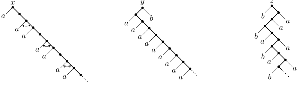
Figure 3: Examples of directed automorphisms x, y, z \in \text{Dir}(\mathcal{T}_d) .
