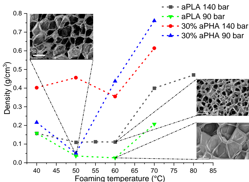
Figure 1 Density and morphology of amorphous PLA foam and an amorphous blend foam containing 30% aPHA at different foaming temperatures and pressures.
