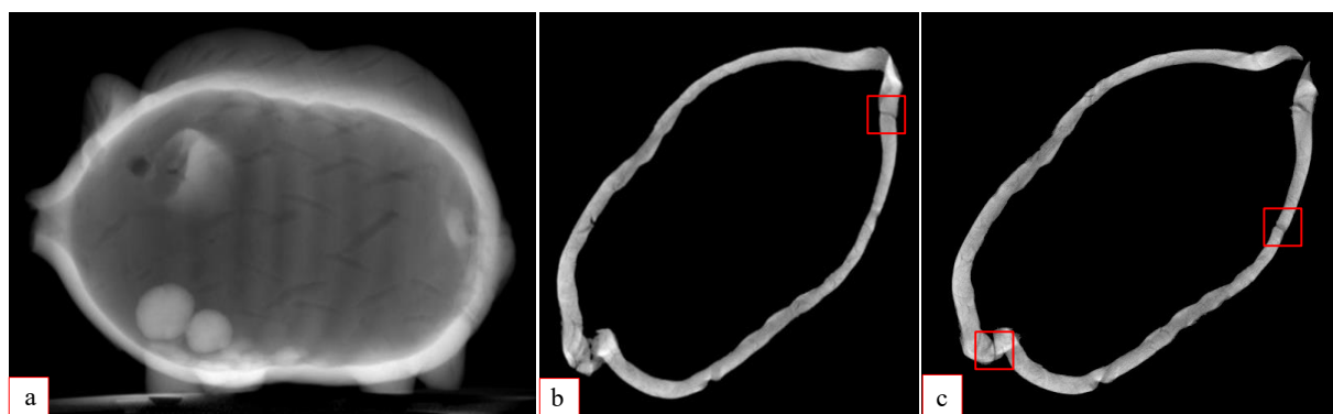
Figure 3. (a) Radiograph of the tintinnabulum; (b) and (c) CT slices where some fractures (red squared) in the ceramic body are visible.
