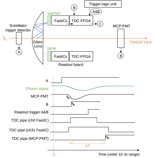
Figure 14. Schematic of the test beam setup. The MCP-PMT signal has a jitter of about 100 ps to the track time. \Delta T is measured between the MCP-PMT and the photon signals from the FastIC using the TDC-in-FPGA. This simplified logic timing diagram does not represent the true signal delays and jitters.
