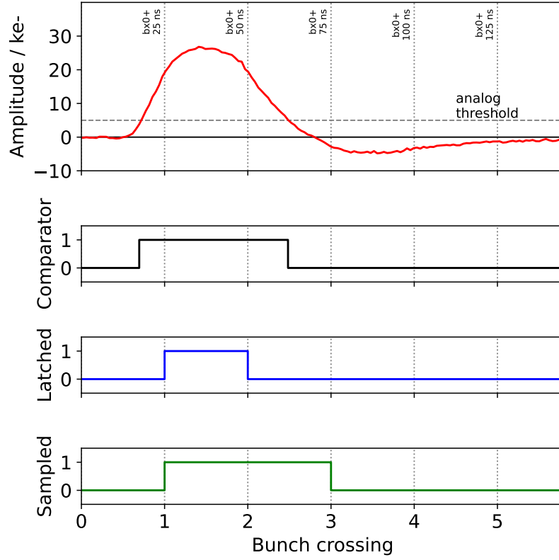
Figure 8. Comparison of the different hit detection modes. The top panel shows the analog pulse reconstructed from a single charge-injected pulse. The pulse height is approximately 25 000 e^- . Applying a threshold leads to a digital comparator output signal, which is converted differently by the latched and the sampled hit detection modes.
