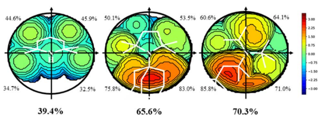
Fig. 1 Topographic steric maps ( xy plane) and % V_{\text{Bur}} of the amines 3 (left), 28 (middle), and 36 (right). The center is on the Z axis, where the Au–N bond would be, specifically at 2.0 \text{ \AA} from N, and the XY plane contains the plane that best defines the 3 N-coordinated atoms. The isocontour curves of the steric maps are given in \text{\AA} . The radius of the sphere around the center was set to 3.5 \text{ \AA} , while for the atoms we adopted the Bondi radii scaled by 1.17, and a mesh of 0.1 \text{ \AA} was used to scan the sphere for buried voxels (the isocontour curves of the steric maps are given in \text{\AA} ).
