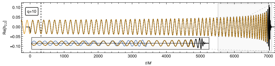
Fig. 7 1PA GSF waveform for a quasicircular, nonspinning binary with mass ratio q = 10 (orange). The inset shows a zoomed portion of the waveform near the merger. Also included for comparison are the 0PA GSF waveform (blue, inset only) and the waveform for the same binary produced using an NR simulation in the SXS catalog (Boyle et al. 2019) (SXS:BBH:1107, in black). The three waveforms are aligned in time and phase at t = 320M , when the orbital separation is \approx 13.83M . Image reproduced from Wardell et al. (2023)
