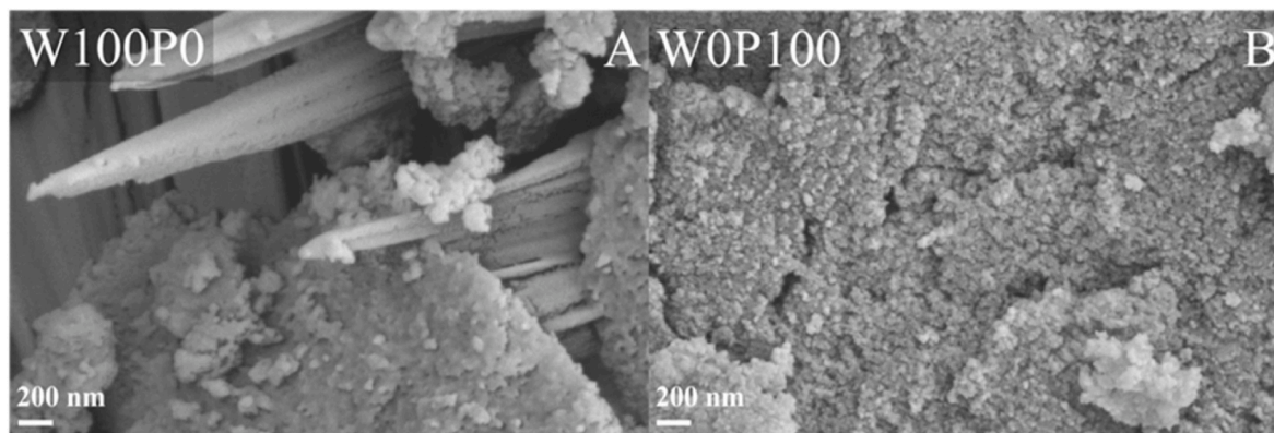
Fig. 2. SEM micrographs of iron oxide-based samples obtained in pure water environment, W100P0 (A, left), and pure 2-propanol environment, WOP100 (B, right). Micrographs were collected at 75k\times magnifications.
