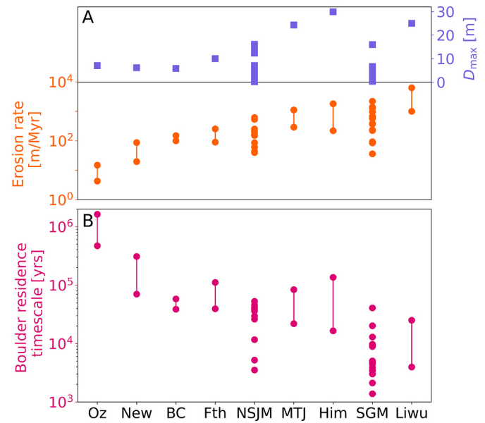
Fig. 2. A) Maximum observed grain sizes ( D_{\max} ) and erosion rates from studies cited below. Oz: Ozarks, Arkansas, USA (Thaler and Covington, 2016; Beeson et al., 2017). New: New River, central Appalachians, Virginia, USA (Granger et al., 1997; Ward et al., 2005; Chilton and Spotila, 2020). BC: Boulder Creek, Colorado, USA (Schildgen et al., 2002; Dühnforth et al., 2012; Dethier et al., 2014; Shobe et al., 2016). Fth: Feather River, Sierra Nevada, USA (Hurst et al., 2012; Attal et al., 2015; Attal, 2017). Low erosion rates from “relict” uplands in the Feather basin are excluded because the largest boulders are observed in “adjusted” channel reaches (Attal et al., 2015; Attal, 2017). NSJM: Northern San Jacinto Mountains, California, USA (Neely et al., 2019; Neely and DiBiase, 2020). MTJ: Mendocino triple junction, northern California, USA (Balco et al., 2013; Roering et al., 2015; Shobe et al., 2020). Him: Nepal Himalaya (Godard et al., 2014; Huber et al., 2020). SGM: San Gabriel Mountains, California, USA (Neely et al., 2019; Neely and DiBiase, 2020). Liwu: Liwu River, Taiwan (Derrieux et al., 2014; Nativ et al., 2019). Erosion rates are the minimum and maximum for each area except for landscapes with paired erosion rate and grain size measurements available (NSJM and SGM; Neely and DiBiase, 2020). B) Boulder residence timescale calculated by dividing D_{\max} by the erosion rate.
