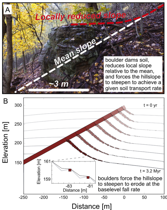
Fig. 5. A) A boulder damming soil on Gap Mountain, Virginia (modified from Fig. 4C in Chilton and Spotila (2020)). B) Numerical simulations of boulder-mantled hillslope evolution showing the development of a quasi-steady-state hillslope (modified from Fig. 3 in Glade et al. (2017)). In this simulation, boulders are released from a dipping, resistant rock layer. The landform achieves a steady-state form with respect to the retreating source of boulders. Boulders increase hillslope steepness and relief by reducing the bedrock weathering rate beneath boulders and by inhibiting soil transport (inset in B) as shown in A). The hillslope is concave-up due to the downslope-fining boulder size distribution that results in greater boulder-induced steepening closer to the hilltop.
