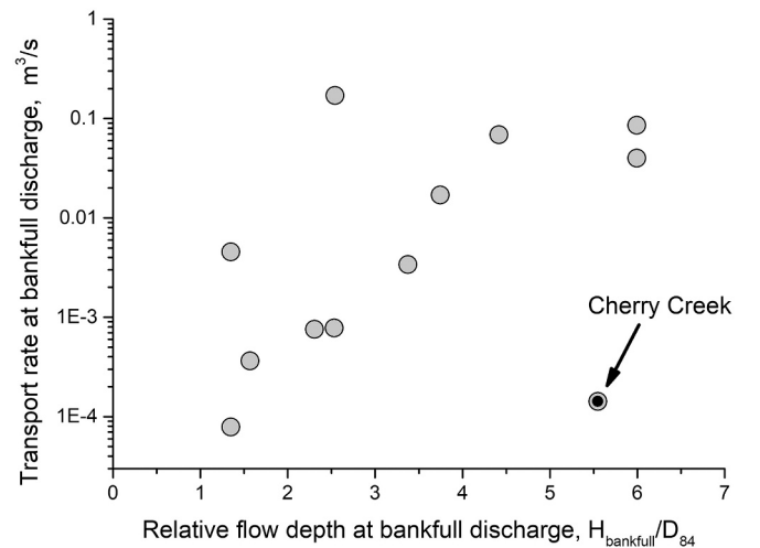
Fig. 8. Bedload transport rate at bankfull discharge as a function of the corresponding relative flow depth, defined as the ratio between bankfull flow depth and the representative grain size D_{84} , in the streams measured by Bunte and Swingle (2021) using bedload traps. This compilation includes streams mainly from the mountains of Colorado, USA, but also includes two sites in the Gros Ventre Range, Wyoming, USA, and one site from the Cascade Range, OR, USA. All else equal, increased relative roughness due to the presence of boulders decreases bedload transport. At Cherry Creek (marked), flow depth was measured in a pool upstream of the sampling site where the flow is much deeper than at the location of the bedload traps.
