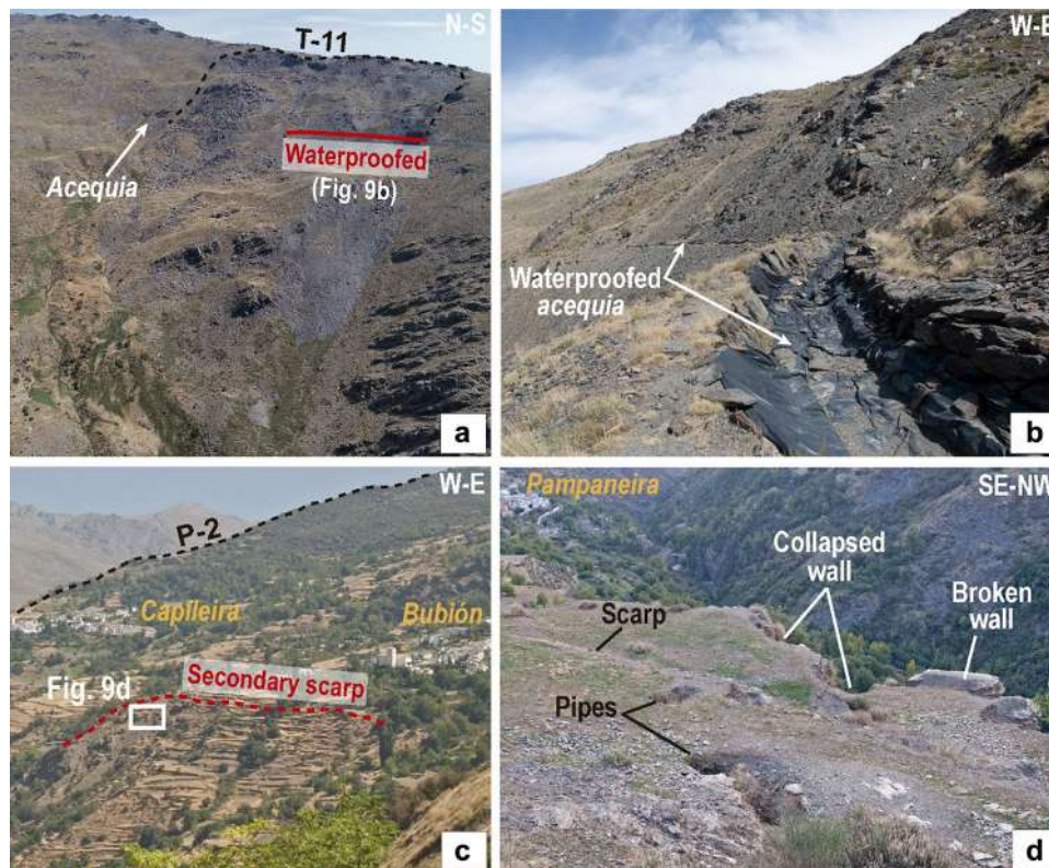
Fig. 9 a Panoramic photograph of the Trevéz-11 (T-11) Landslide. Its main scarp is drawn by a black-coloured dashed line. An acequia de careo , which runs across the landslide, and its waterproofed transect are also indicated. b Detail of the waterproofed transect (black-coloured plastic) of the acequia de careo . c Lateral view of a secondary (or nested) movement and its scarp within the Poqueira-2 (P-2) Landslide. The villages of Capileira and Bubión are also indicated. d Damages of terraced fields within the nested body of the Poqueira-2 Landslide. Piping phenomena, minor scarps and damaged dry walls are evidences of the active ground movement. The village of Pampaneira is also indicated
