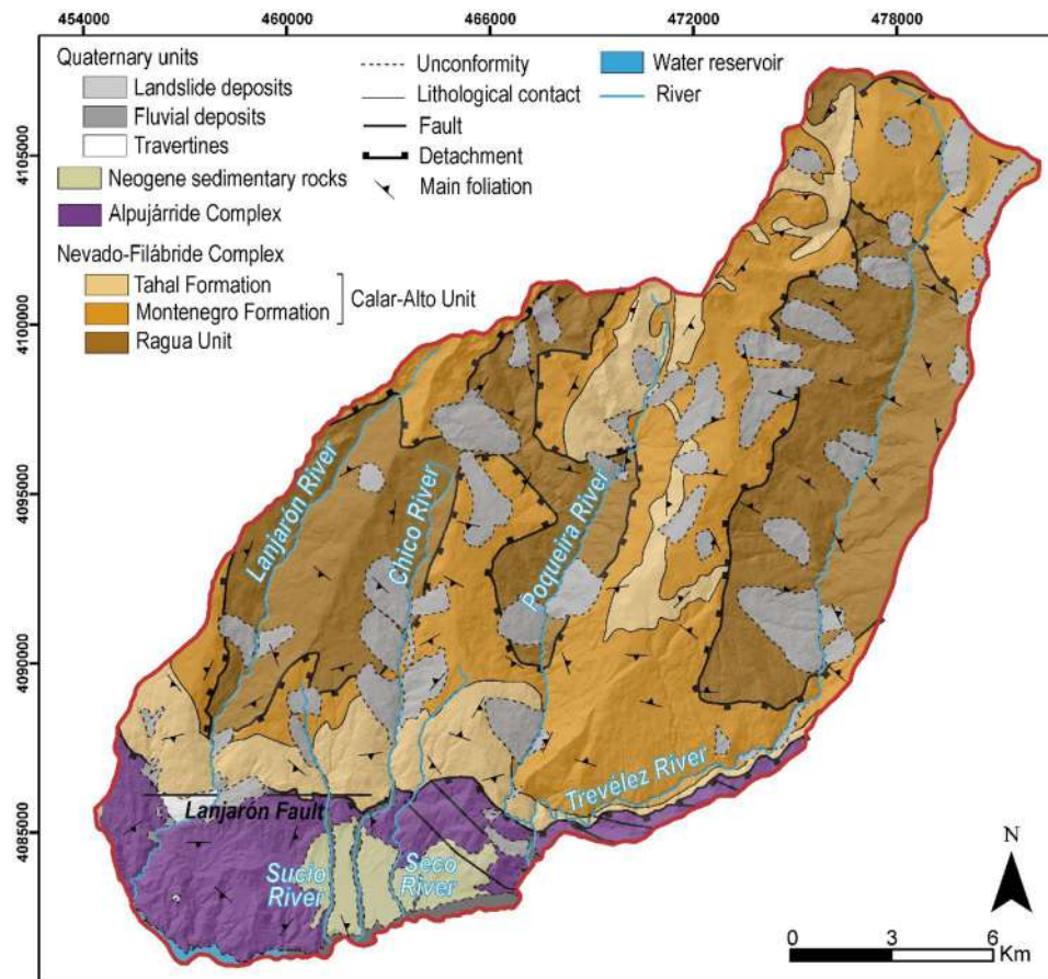
Fig. 2 Geological map of the study area, modified from Azañón et al. (2015). The analysed rivers (from west to east) of Lanjarón, Sucio, Chico, Seco, Poqueira and Trevélez are also indicated. The slope movements are those included in the Spanish Land Movements Database (BD-MOVES). The Lanjarón Fault is a probably active fault, according to Sanz de Galdeano et al. (2003), which is also included in the Quaternary Active Faults Database of Iberia (QAFI)
